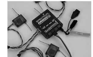
Shown using a separate receiver pack. (Battery can be plugged into either BATT port.)
